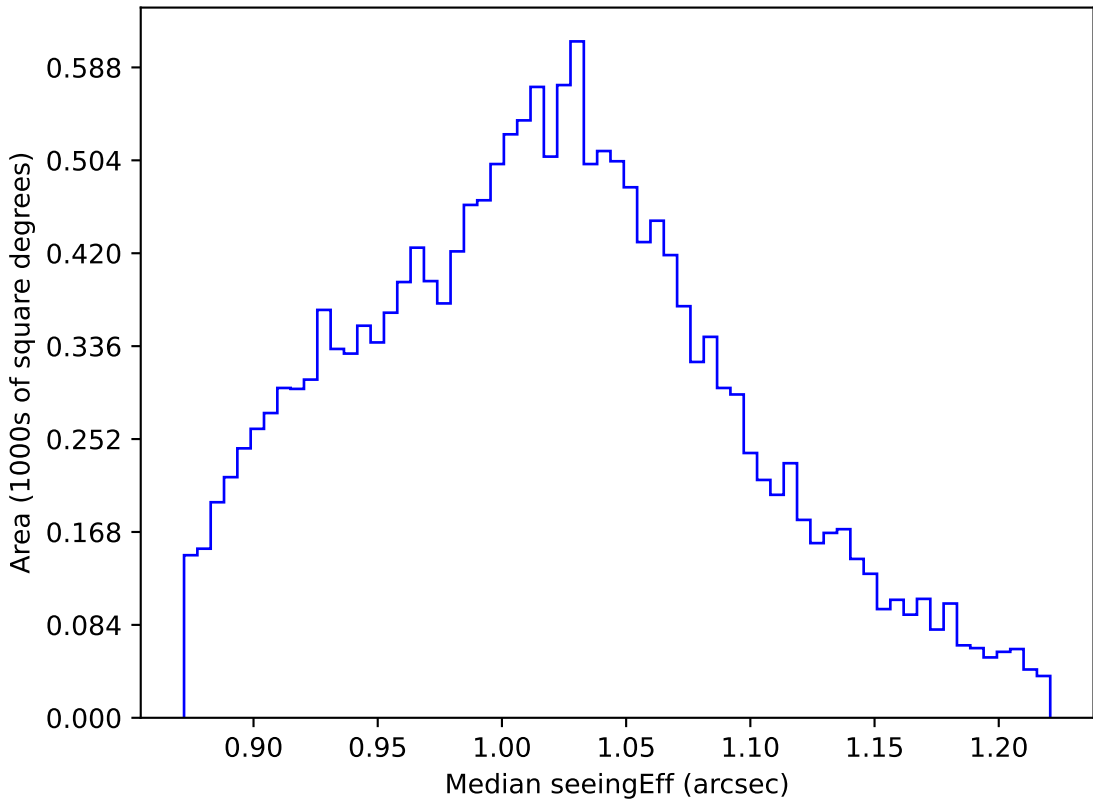
weather_cloudso14v3.4_10yrs WFD i band: Median seeingEff
