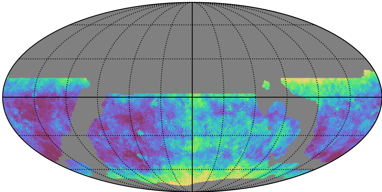
weather_cloudso14v3.4_10yrs WFD g band: Median seeingEff
