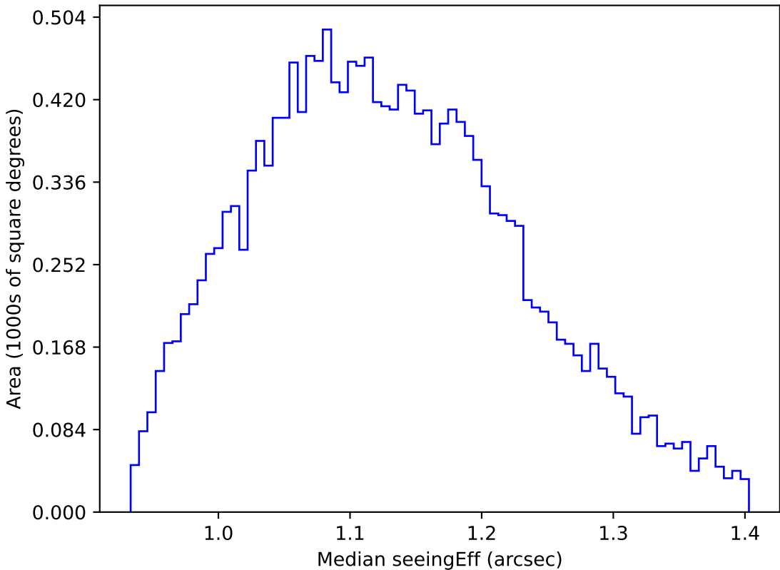
weather_cloudso14v3.4_10yrs WFD g band: Median seeingEff
