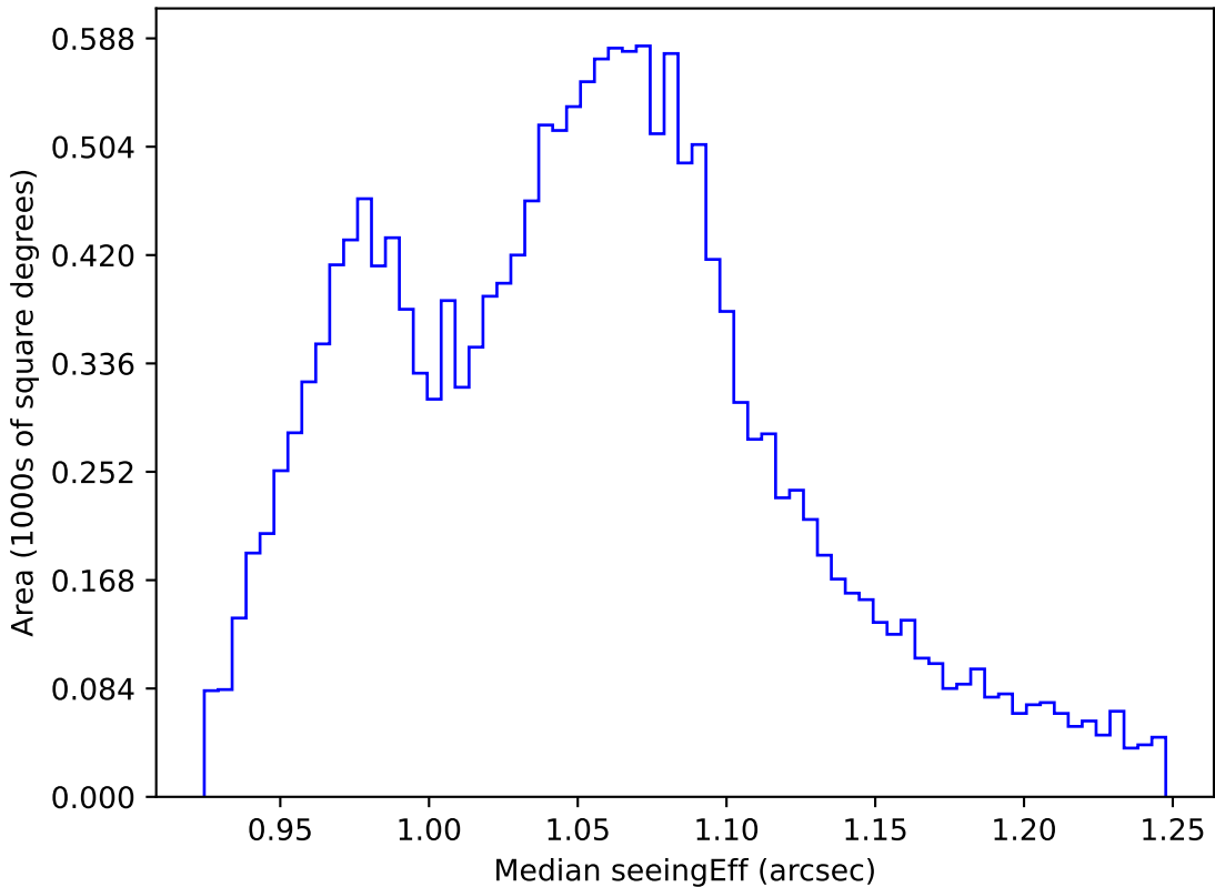
weather_cloudso14v3.4_10yrs WFD all bands: Median seeingEff
