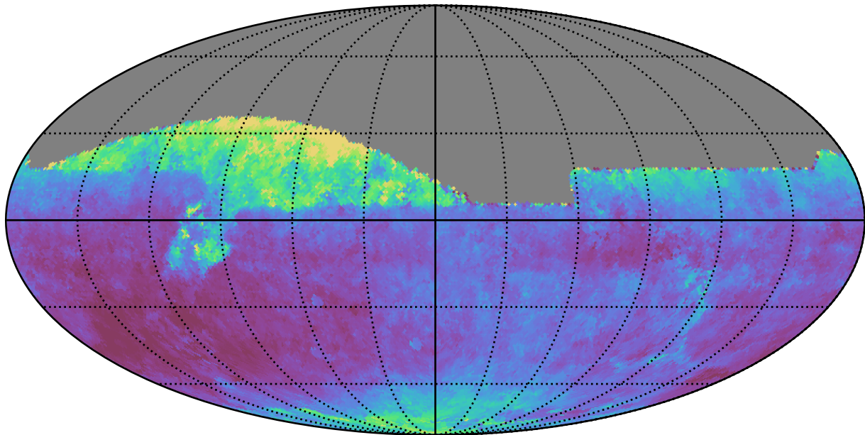
weather_cloudso14v3.4_10yrs All sky z band: Median seeingEff
