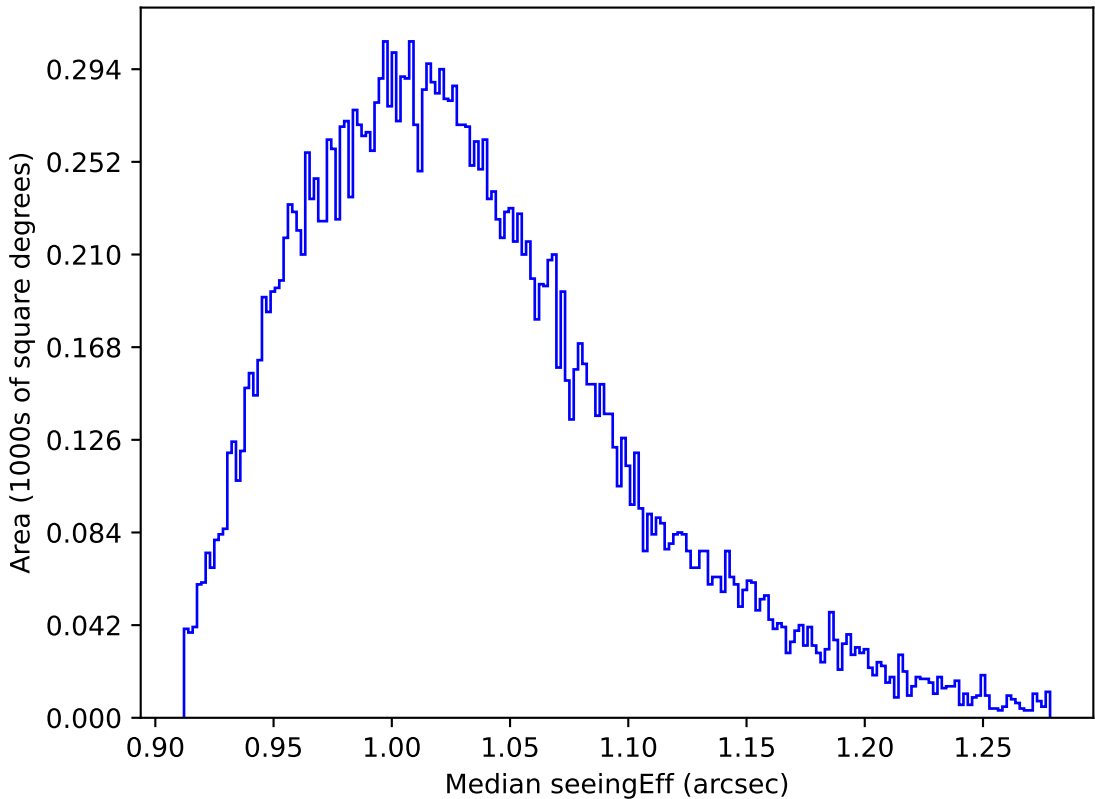
weather_cloudso14v3.4_10yrs All sky y band: Median seeingEff
