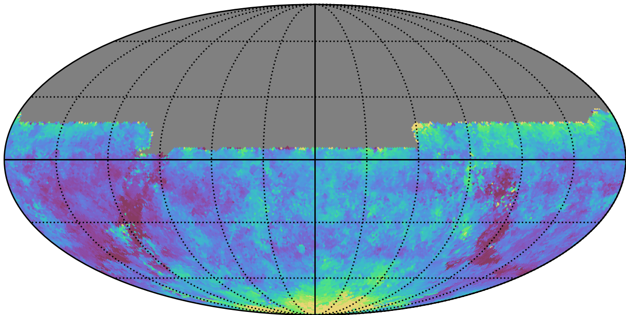
weather_cloudso14v3.4_10yrs All sky u band: Median seeingEff
