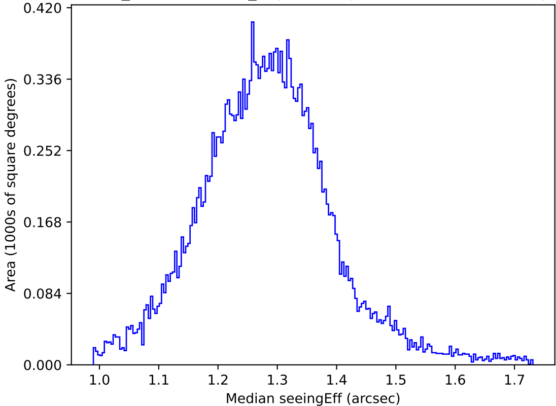
weather_cloudso14v3.4_10yrs All sky u band: Median seeingEff
