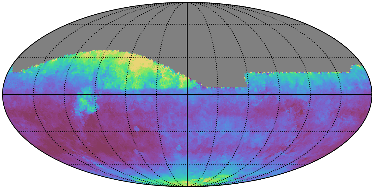
weather_cloudso14v3.4_10yrs All sky i band: Median seeingEff
