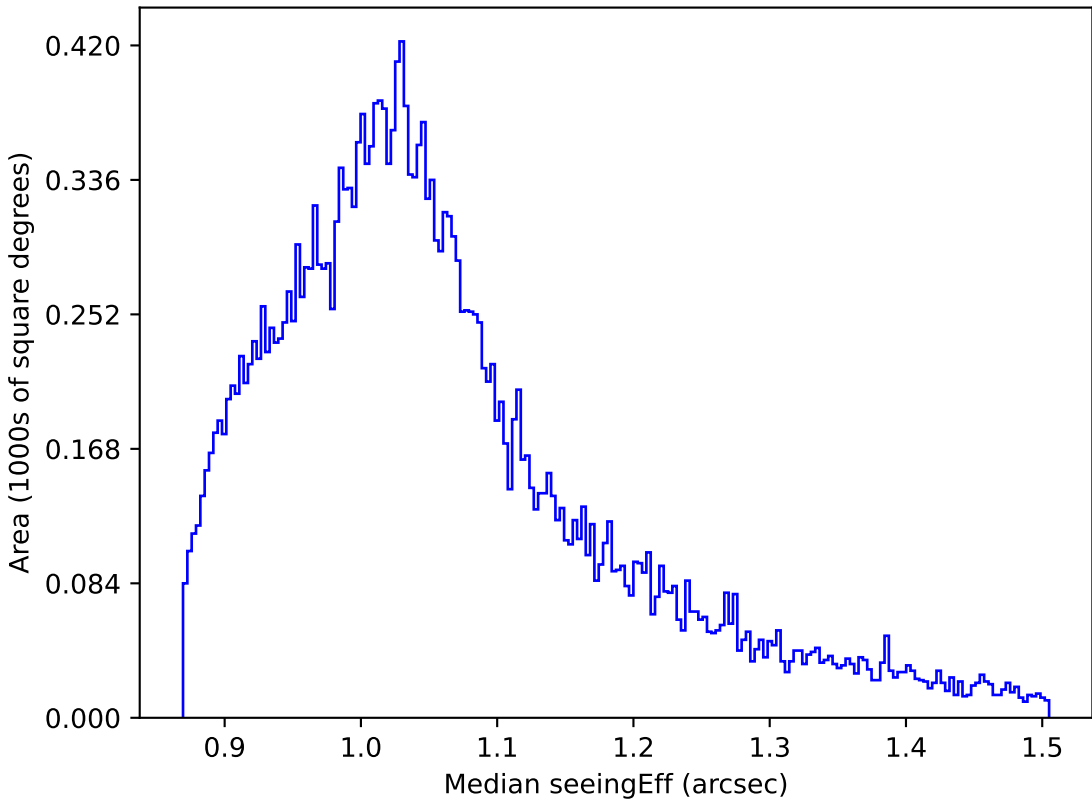
weather_cloudso14v3.4_10yrs All sky i band: Median seeingEff
