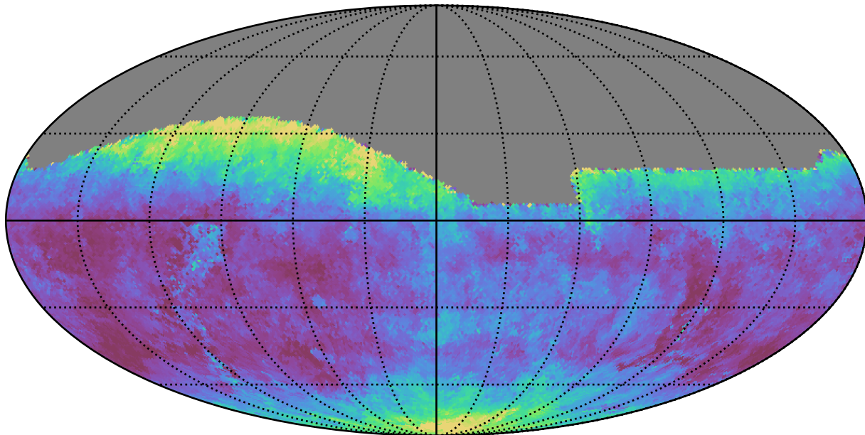
weather_cloudso14v3.4_10yrs All sky g band: Median seeingEff
