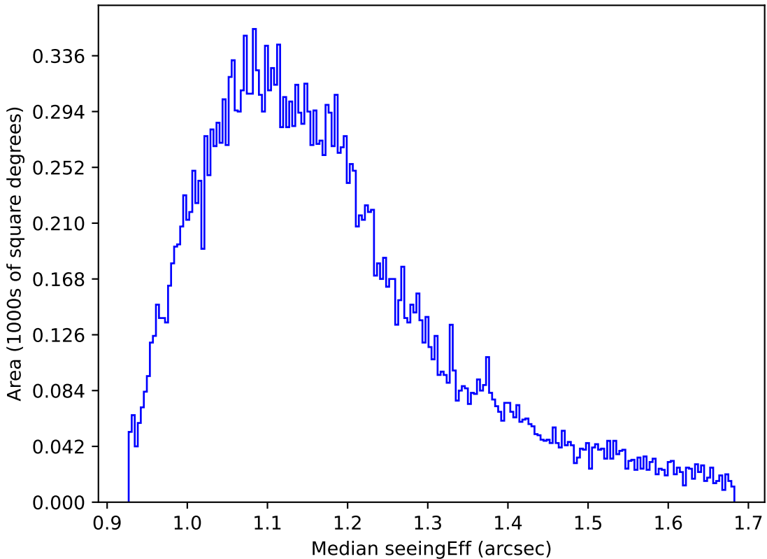
weather_cloudso14v3.4_10yrs All sky g band: Median seeingEff
