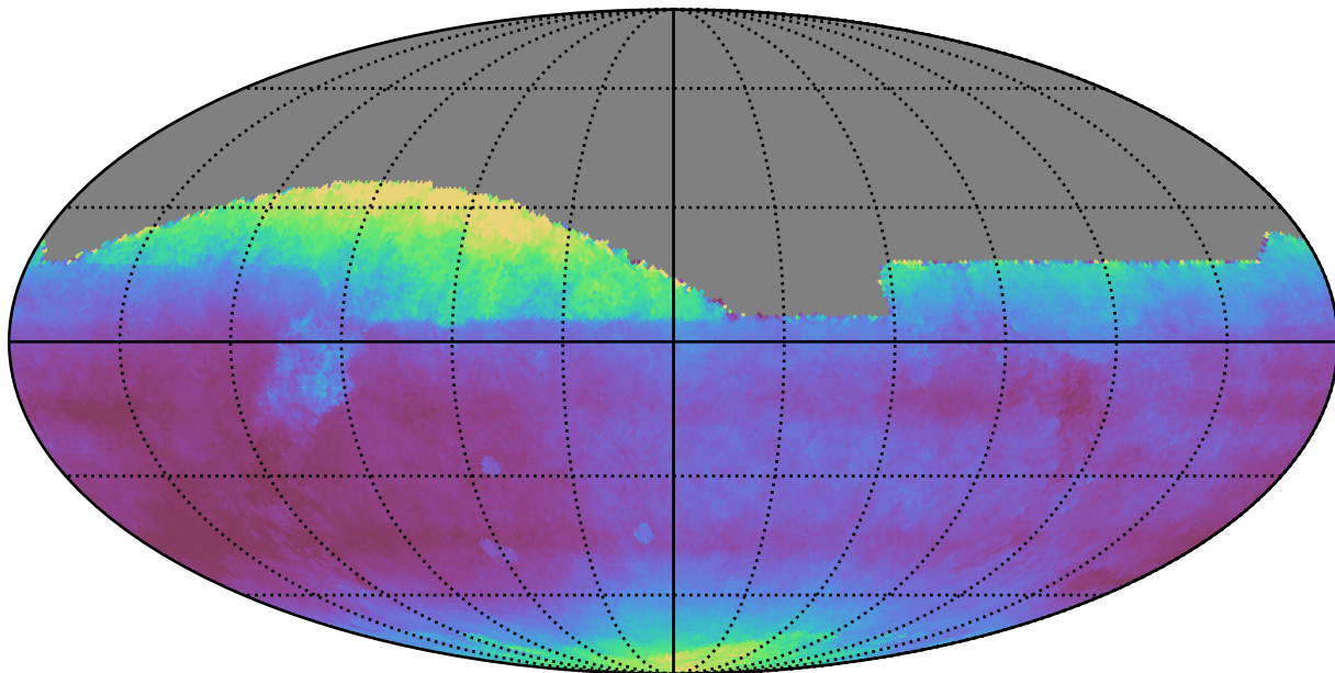
weather_cloudso14v3.4_10yrs All sky all bands: Median seeingEff
