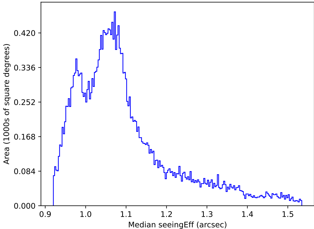
weather_cloudso14v3.4_10yrs All sky all bands: Median seeingEff
