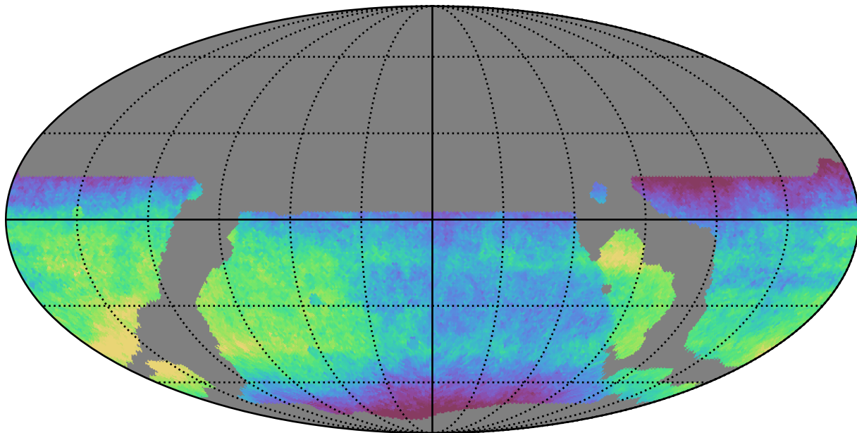
weather_cloudso14v3.4_10yrs WFD all bands: Median saturation_mag
