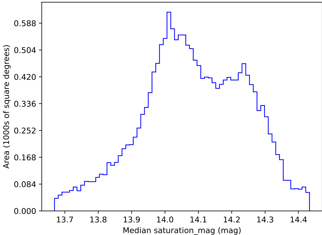
weather_cloudso14v3.4_10yrs WFD all bands: Median saturation_mag
