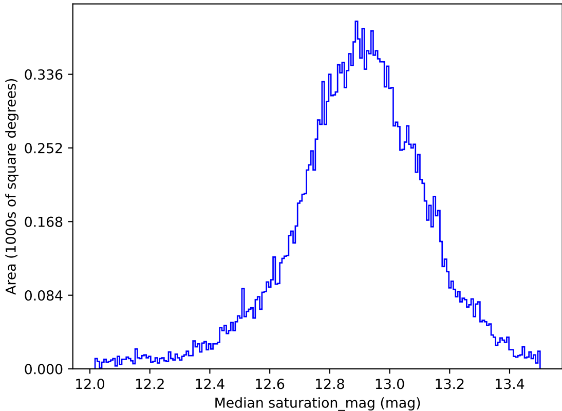
weather_cloudso14v3.4_10yrs All sky u band: Median saturation_mag
