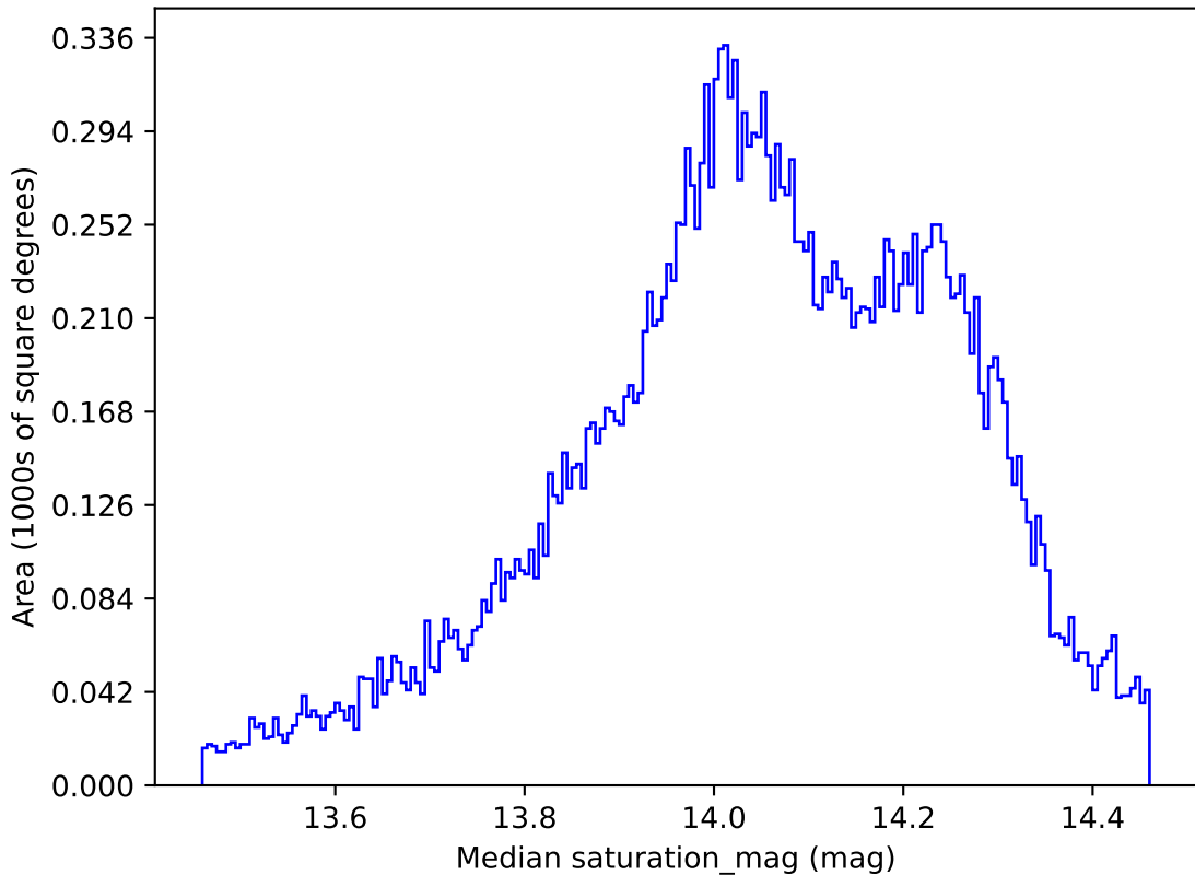
weather_cloudso14v3.4_10yrs All sky all bands: Median saturation_mag
