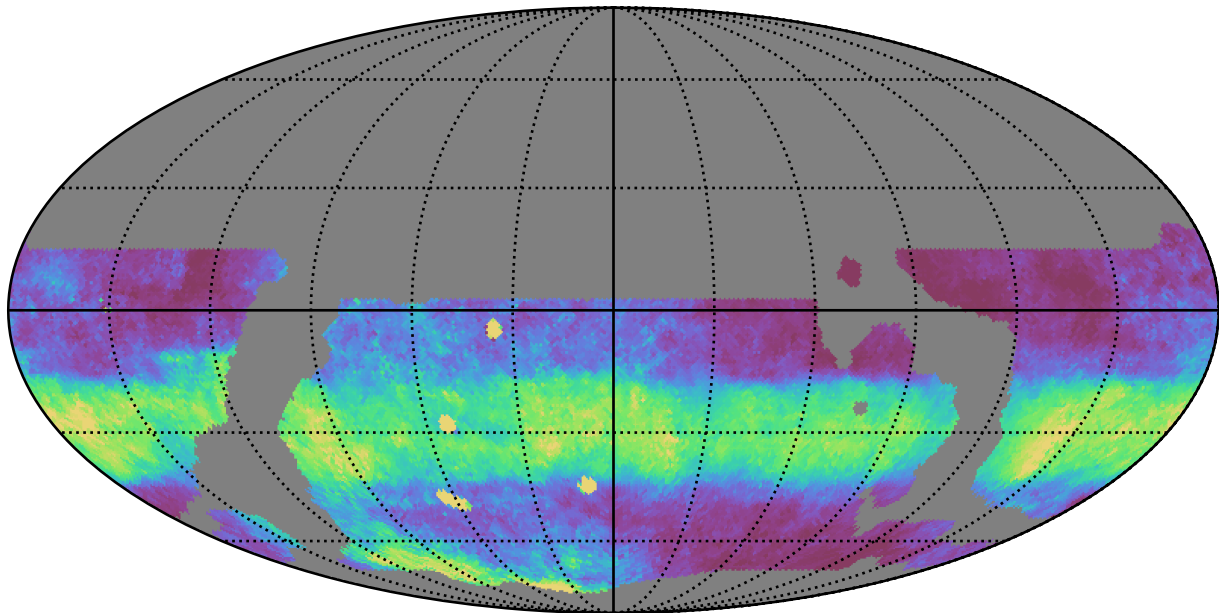
weather_cloudso14v3.4_10yrs WFD z band: Median normairmass
