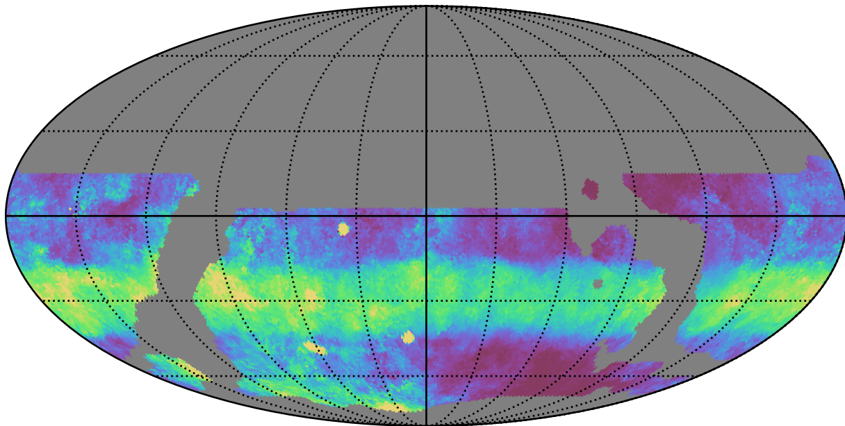
weather_cloudso14v3.4_10yrs WFD y band: Median normairmass
