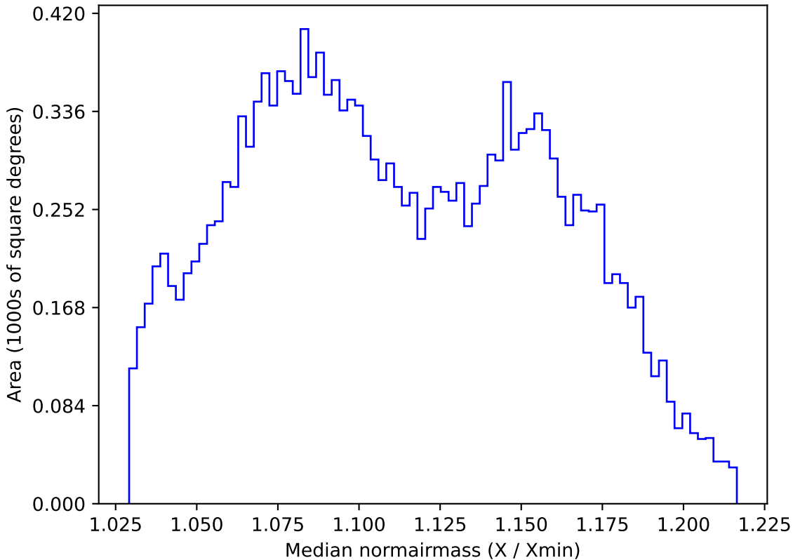
weather_cloudso14v3.4_10yrs WFD y band: Median normairmass
