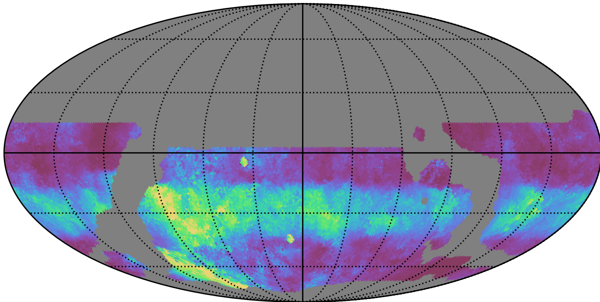
weather_cloudso14v3.4_10yrs WFD u band: Median normairmass
