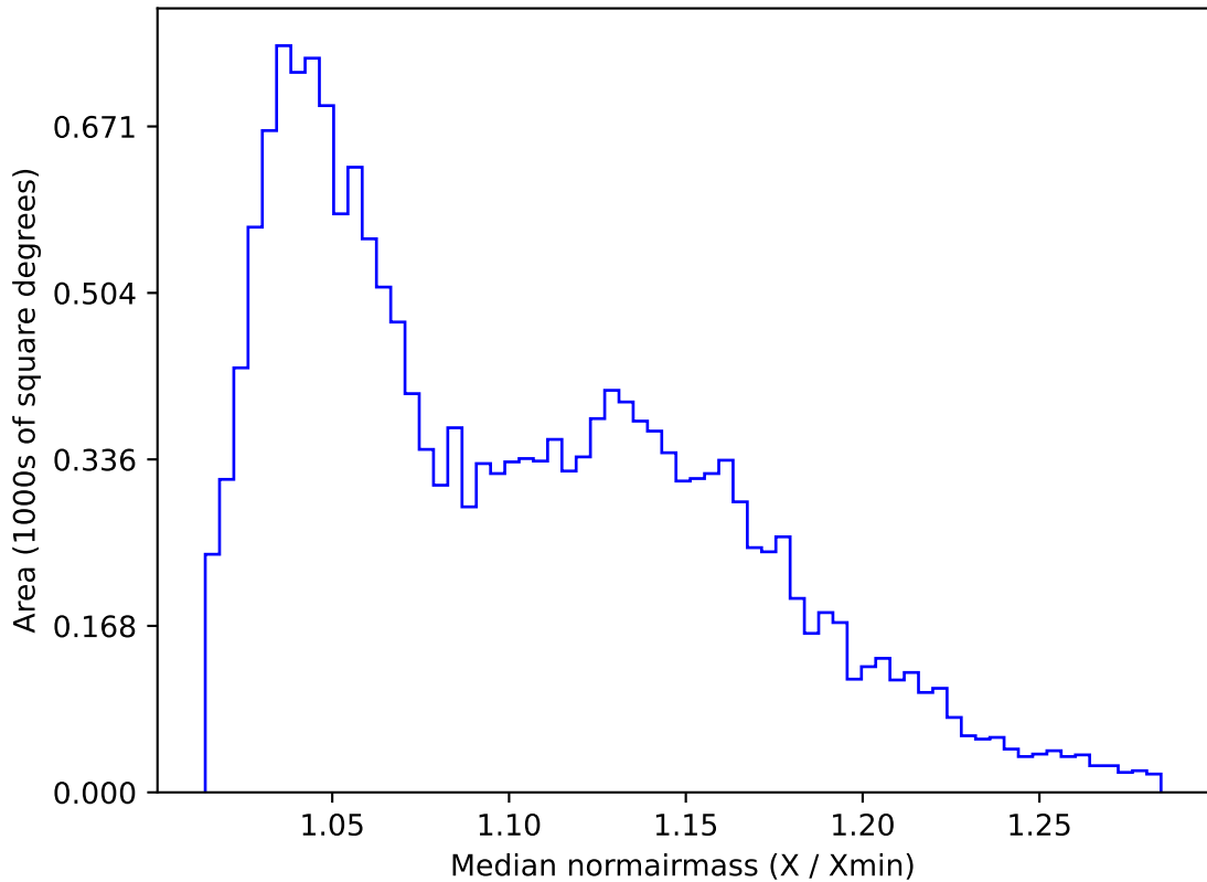
weather_cloudso14v3.4_10yrs WFD u band: Median normairmass
