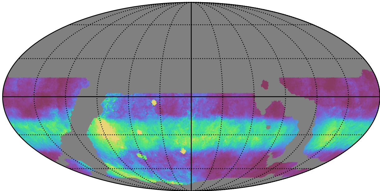
weather_cloudso14v3.4_10yrs WFD r band: Median normairmass
