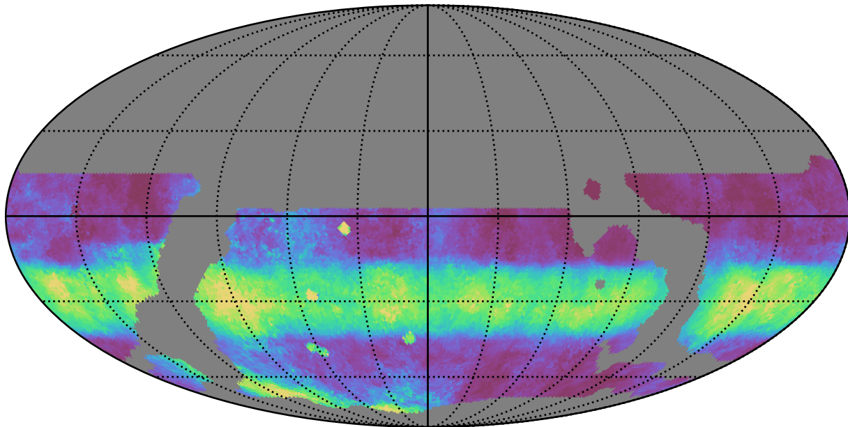
weather_cloudso14v3.4_10yrs WFD i band: Median normairmass
