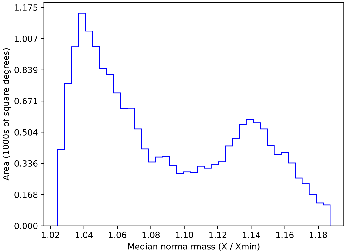
weather_cloudso14v3.4_10yrs WFD i band: Median normairmass
