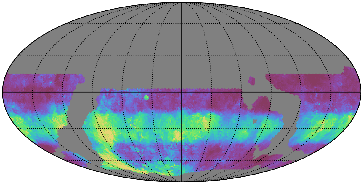
weather_cloudso14v3.4_10yrs WFD g band: Median normairmass
