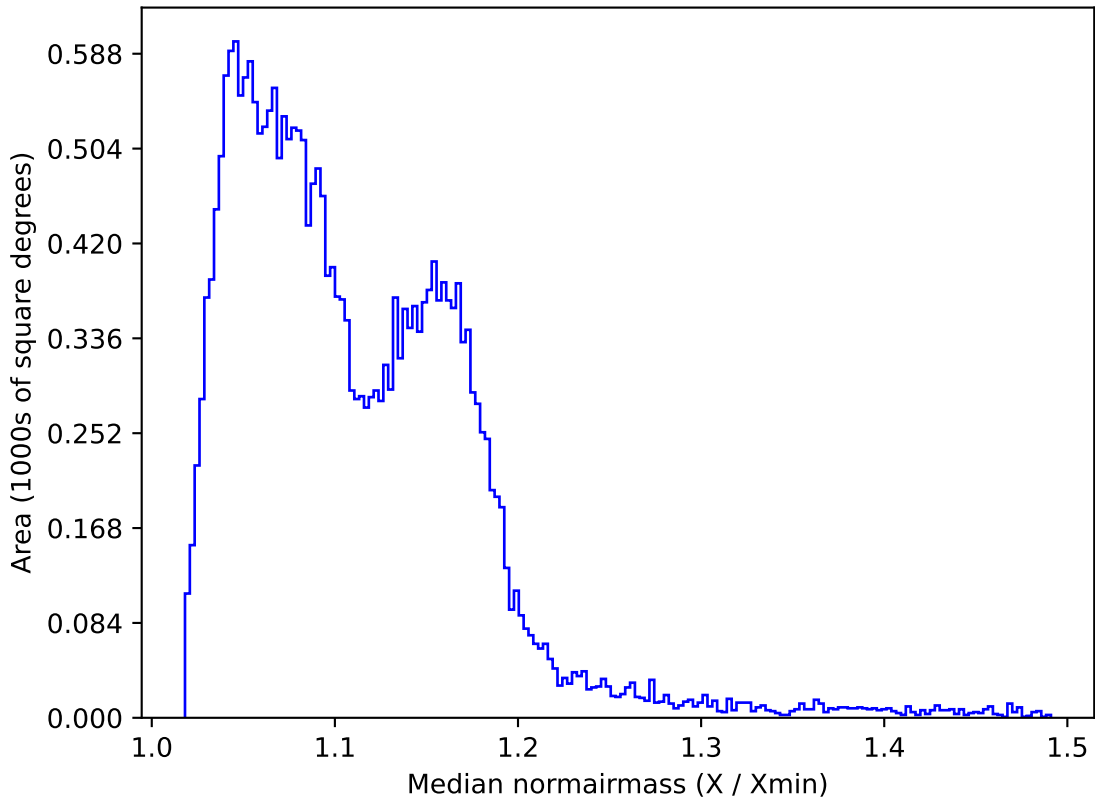
weather_cloudso14v3.4_10yrs All sky z band: Median normairmass
