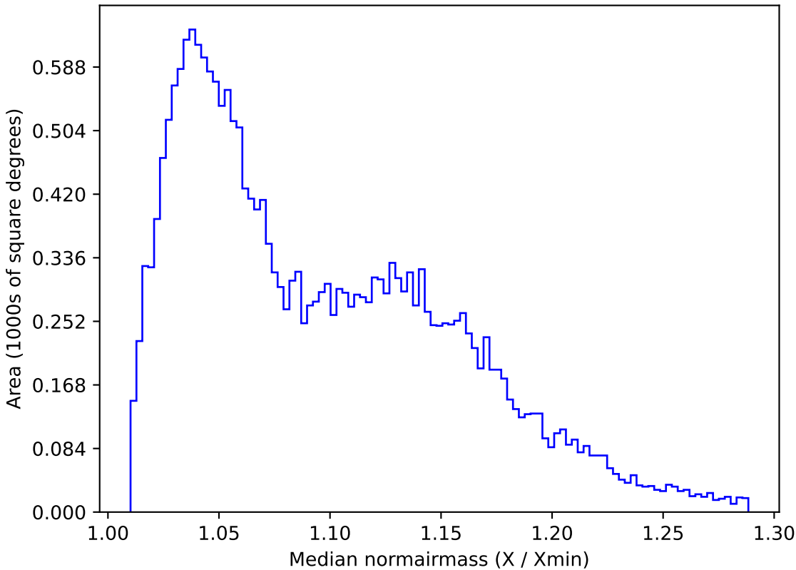
weather_cloudso14v3.4_10yrs All sky u band: Median normairmass
