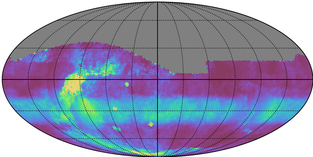
weather_cloudso14v3.4_10yrs All sky r band: Median normairmass
