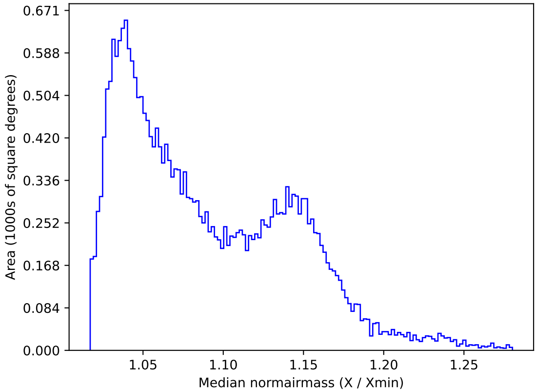
weather_cloudso14v3.4_10yrs All sky r band: Median normairmass
