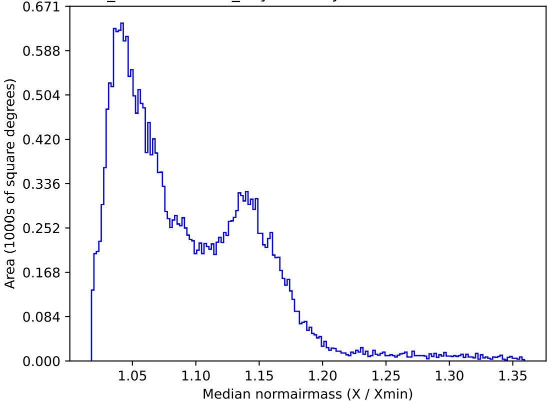
weather_cloudso14v3.4_10yrs All sky i band: Median normairmass
