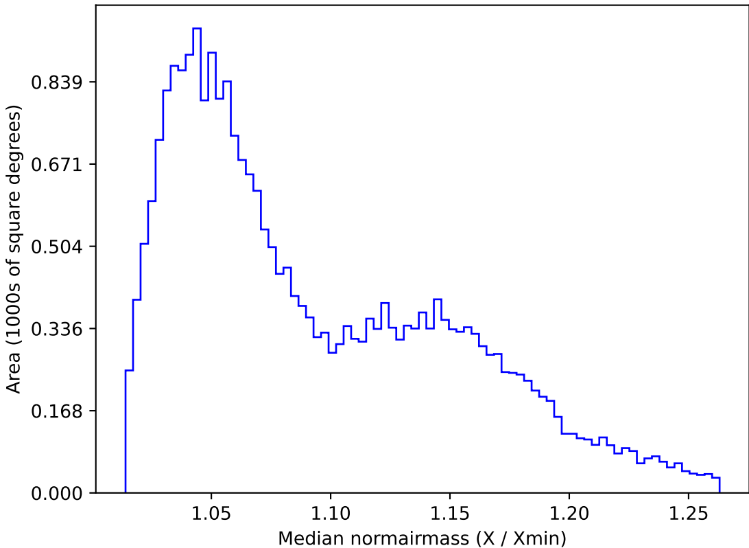
weather_cloudso14v3.4_10yrs All sky g band: Median normairmass
