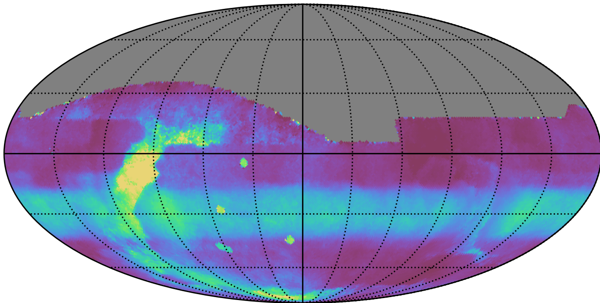
weather_cloudso14v3.4_10yrs All sky all bands: Median normairmass
