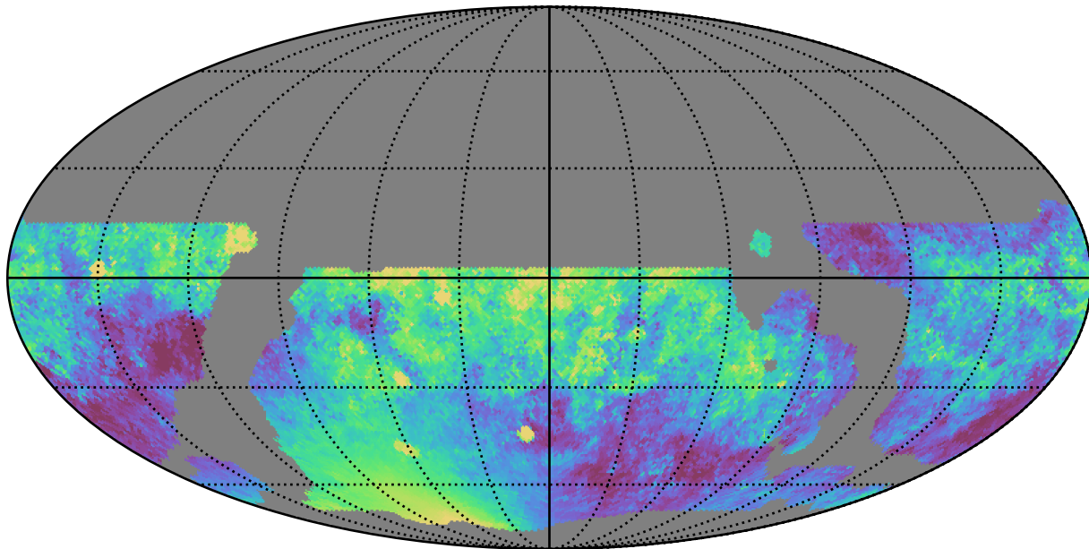
weather_cloudso14v3.4_10yrs WFD z band: Median moonDistance
