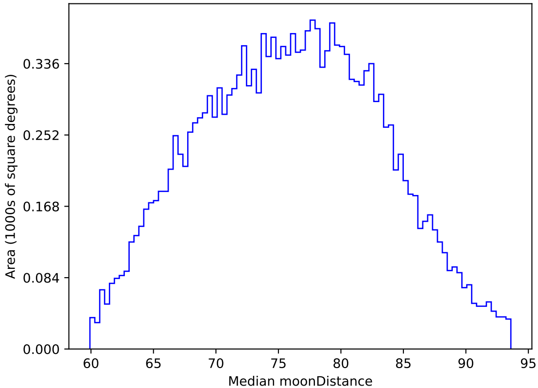
weather_cloudso14v3.4_10yrs WFD z band: Median moonDistance
