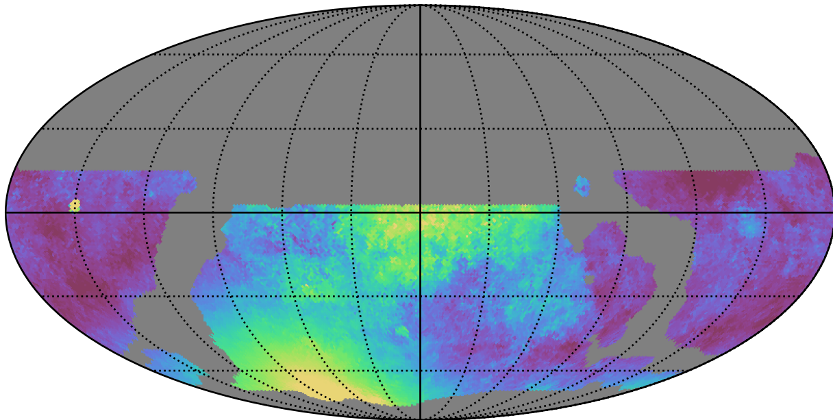
weather_cloudso14v3.4_10yrs WFD y band: Median moonDistance
