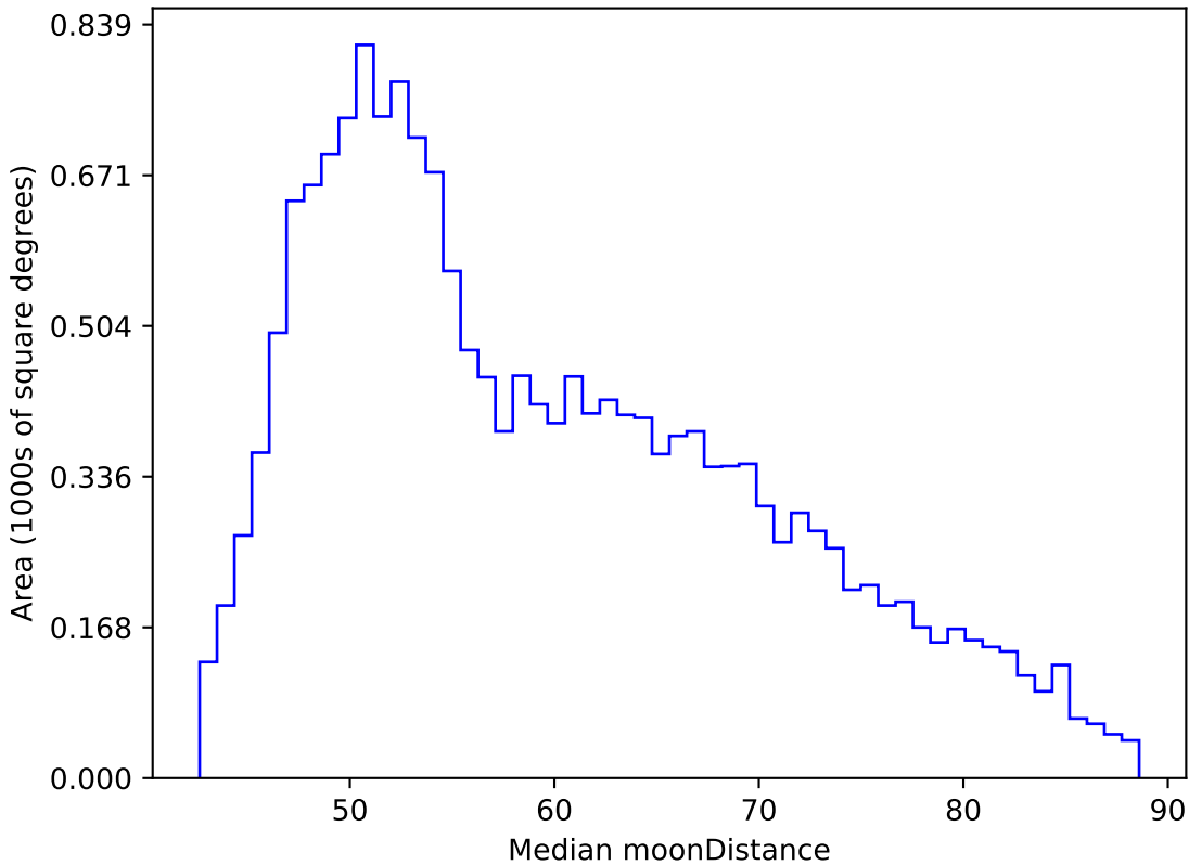
weather_cloudso14v3.4_10yrs WFD y band: Median moonDistance
