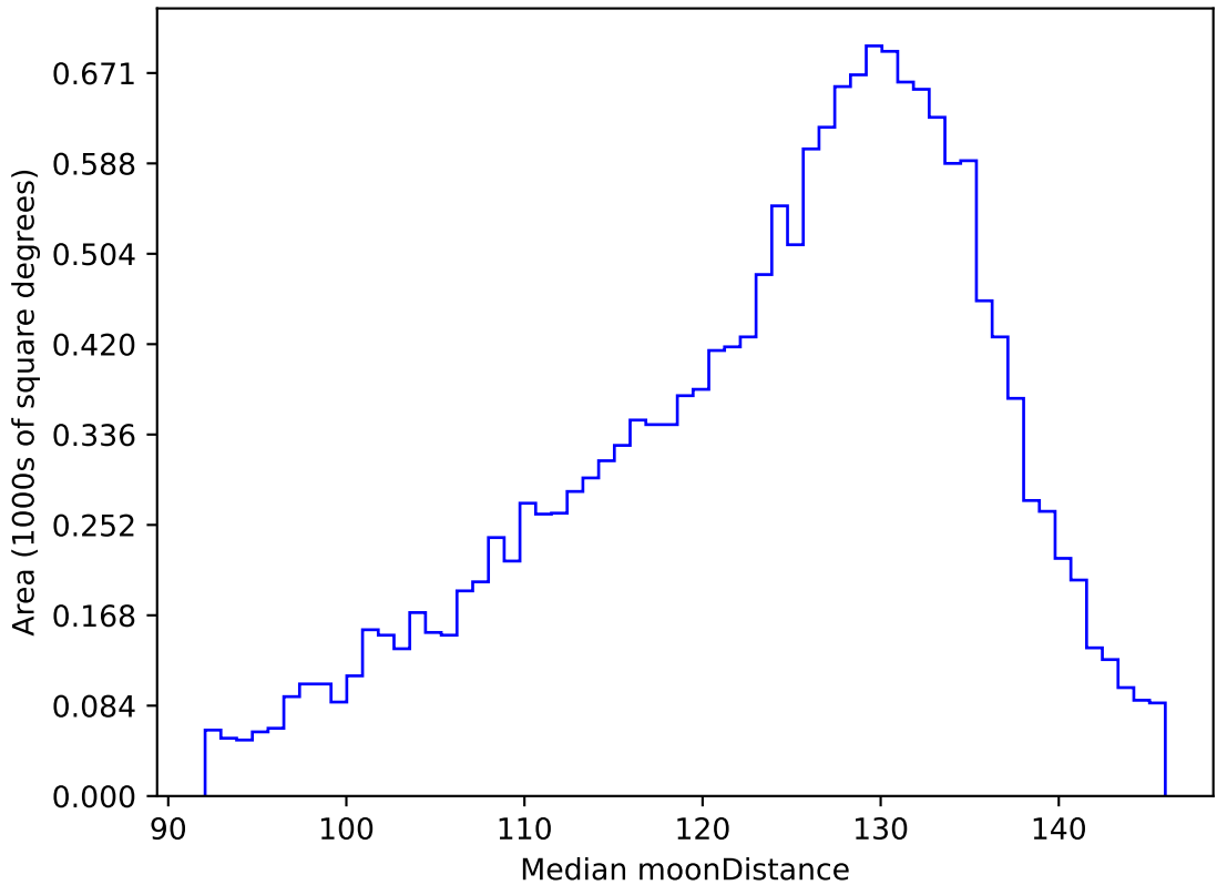
weather_cloudso14v3.4_10yrs WFD u band: Median moonDistance
