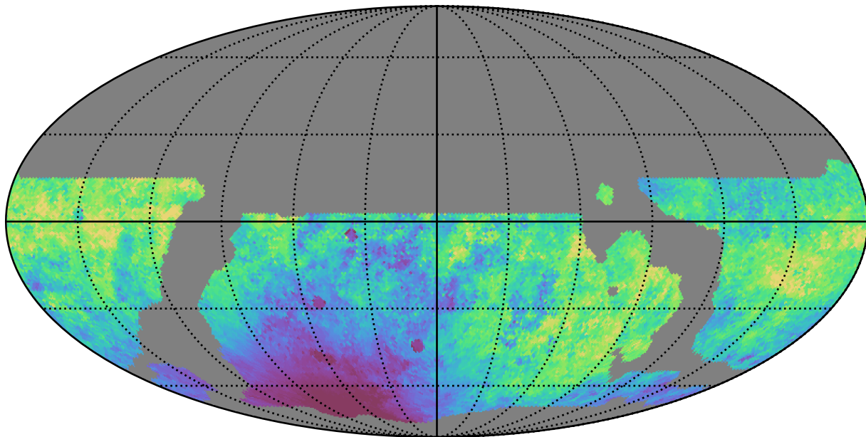
weather_cloudso14v3.4_10yrs WFD r band: Median moonDistance
