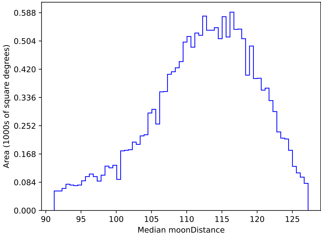
weather_cloudso14v3.4_10yrs WFD r band: Median moonDistance
