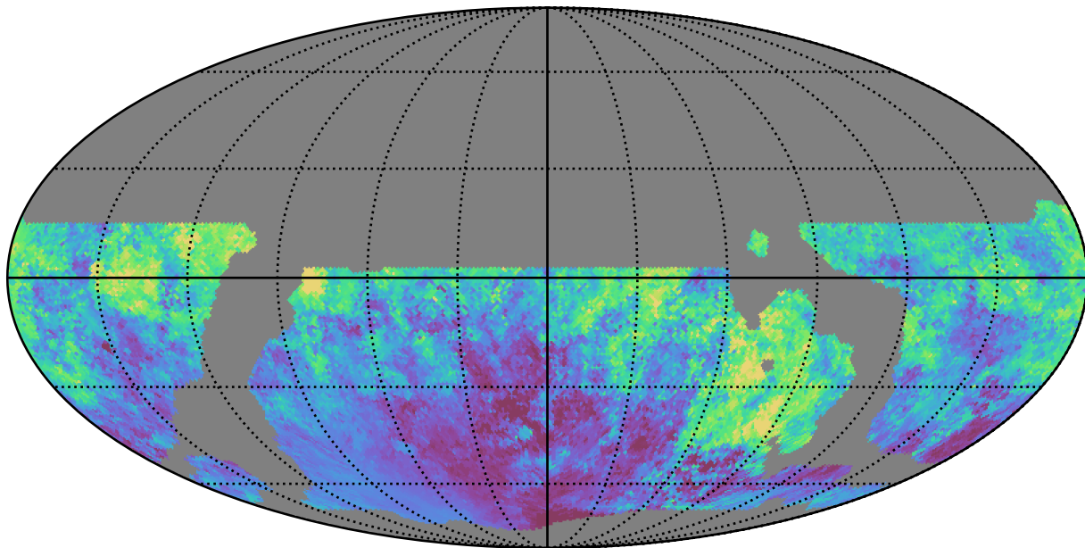
weather_cloudso14v3.4_10yrs WFD i band: Median moonDistance
