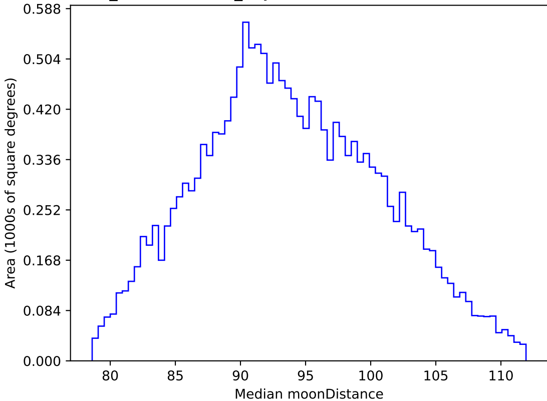
weather_cloudso14v3.4_10yrs WFD i band: Median moonDistance
