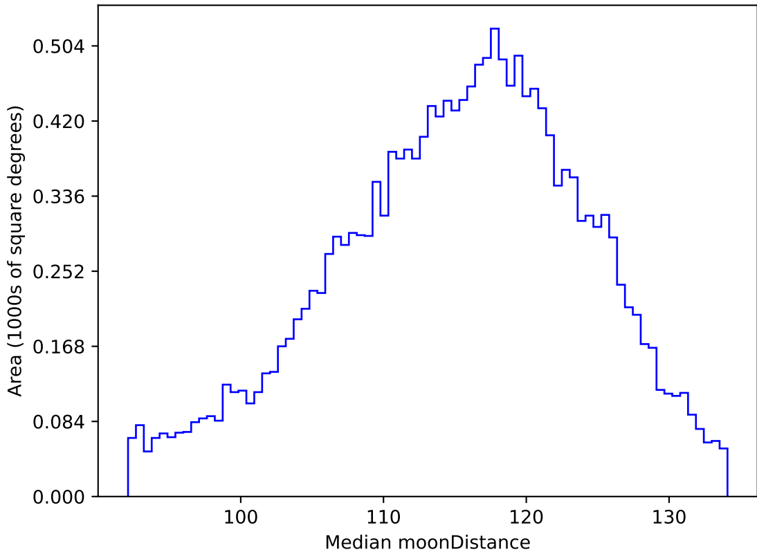
weather_cloudso14v3.4_10yrs WFD g band: Median moonDistance
