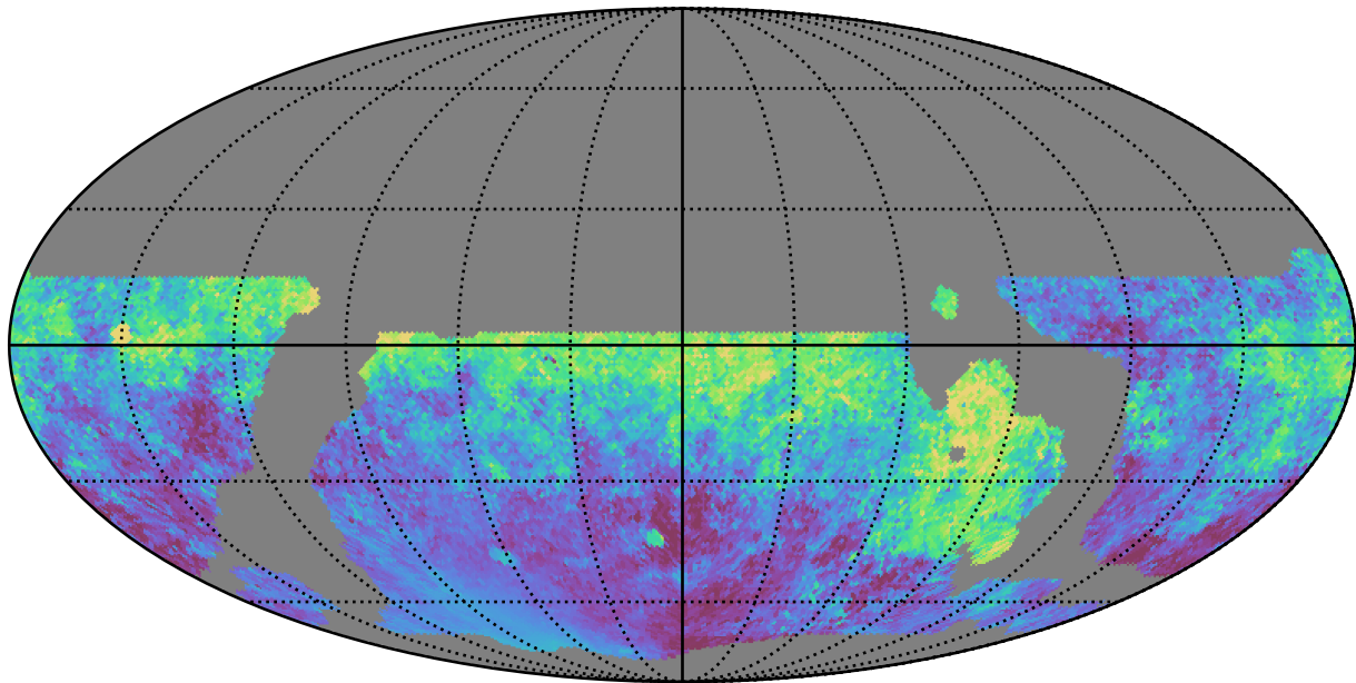
weather_cloudso14v3.4_10yrs WFD all bands: Median moonDistance
