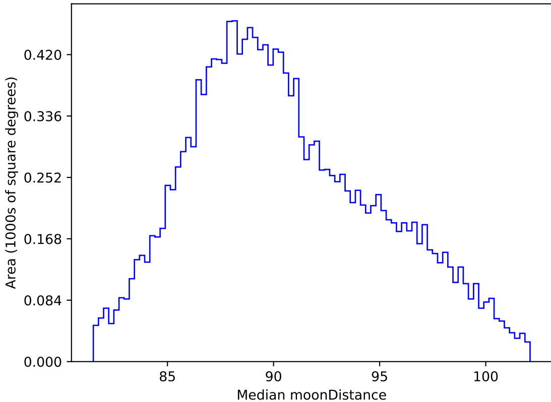
weather_cloudso14v3.4_10yrs WFD all bands: Median moonDistance
