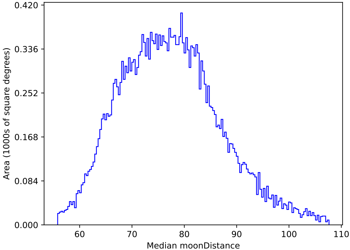
weather_cloudso14v3.4_10yrs All sky z band: Median moonDistance
