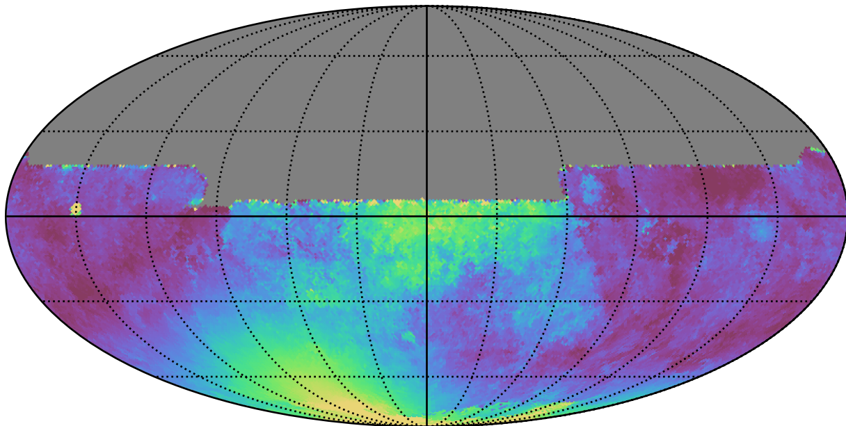
weather_cloudso14v3.4_10yrs All sky y band: Median moonDistance
