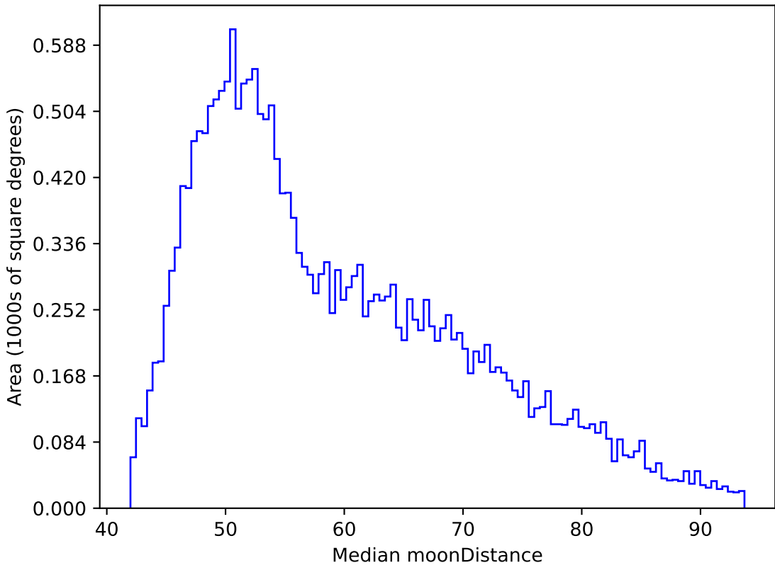
weather_cloudso14v3.4_10yrs All sky y band: Median moonDistance
