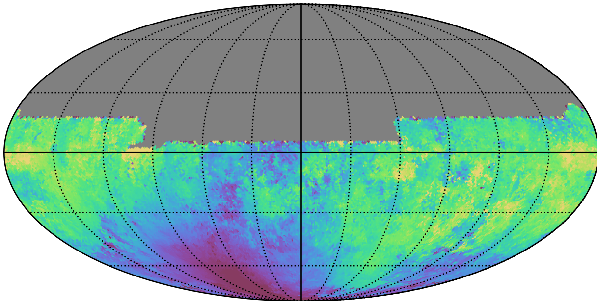
weather_cloudso14v3.4_10yrs All sky u band: Median moonDistance
